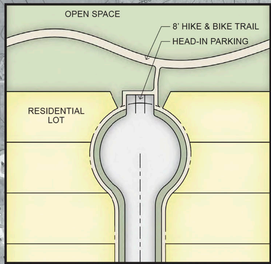
Typical Cul-De-Sac Detail Adjacent to Open Space N.T.S.
